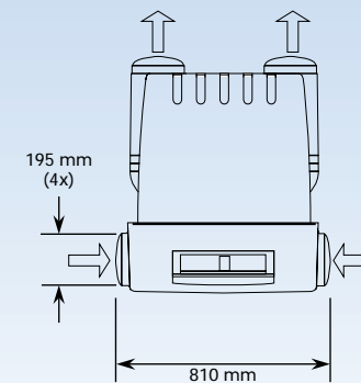
Dimensions Statiflex 200-M
